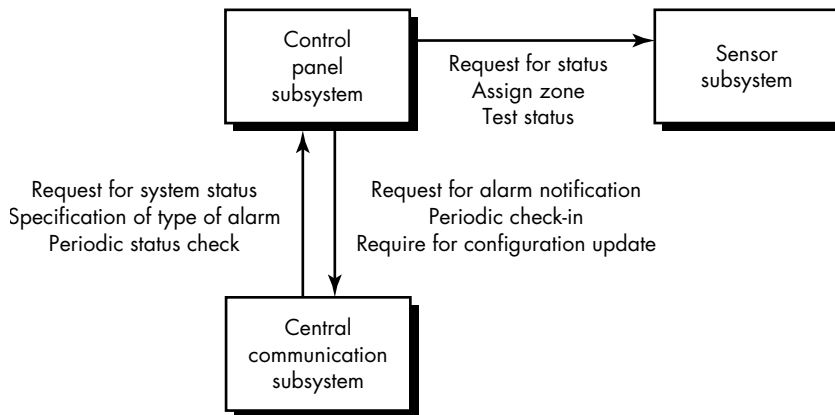
FIGURE 22.6 Abbreviated subsystem collaboration graph for Safe- Home
