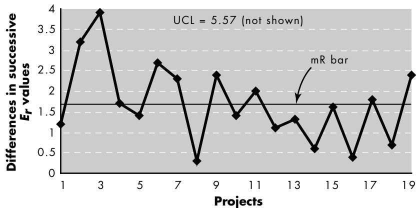
FIGURE 4.9 Moving range control chart
